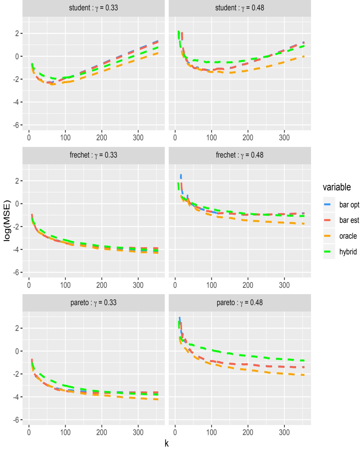
Figure 6: \text{MSE} estimates (in log scale) against k , for Student (top), Fréchet (middle) and Pareto (bottom) distributions, with \gamma = 0.33 (left) and \gamma = 0.48 (right). Results for \bar{\xi}_{\tau'_n}^*(\alpha(\gamma), \beta_{\alpha(\gamma)}(\gamma))/\xi_{\tau'_n} in blue, \bar{\xi}_{\tau'_n}^*/\xi_{\tau'_n} in red, \bar{\xi}_{\tau'_n}^*(1/2, 1/2)/\xi_{\tau'_n} in green, and \bar{\xi}_{\tau'_n}^*(\alpha_{\text{oracle}}, \beta_{\text{oracle}})/\xi_{\tau'_n} in orange.
