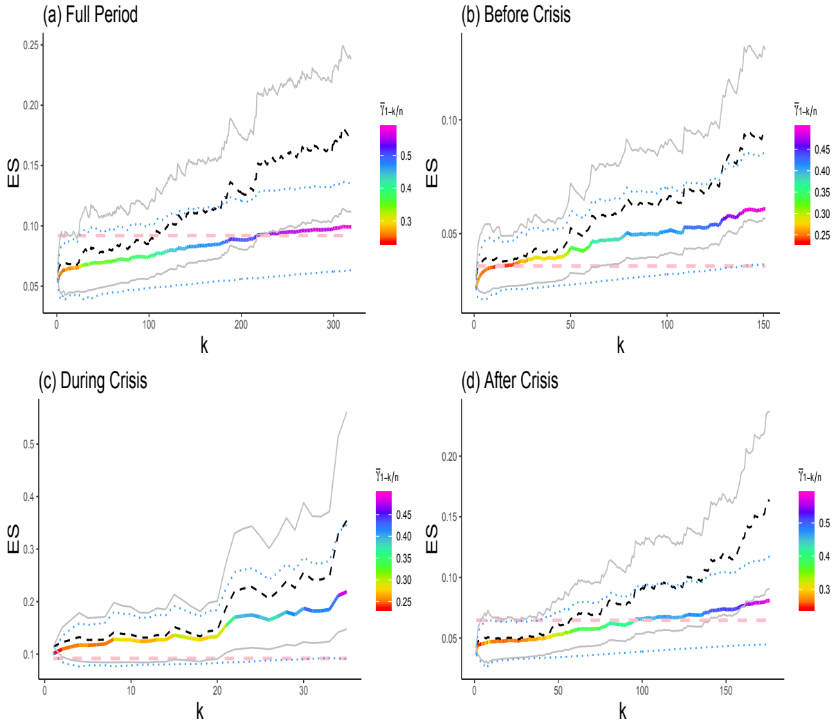
Figure 6: Plots of the ES estimates based on daily loss returns of the SPDR S&P 500 ETF (SPY). The estimates \widehat{XES}_{\hat{\tau}_n^*}^*(p_n) as rainbow curve and \overline{XES}_{\hat{\tau}_n^*}^*(p_n) as dashed black curve, along with the asymptotic 95% confidence intervals \widetilde{CI}_{0.95}(k) in dotted blue lines and \overline{CI}_{0.95}(k) in solid grey lines. The sample maximum Y_{n,n} indicated in horizontal dashed pink line.
