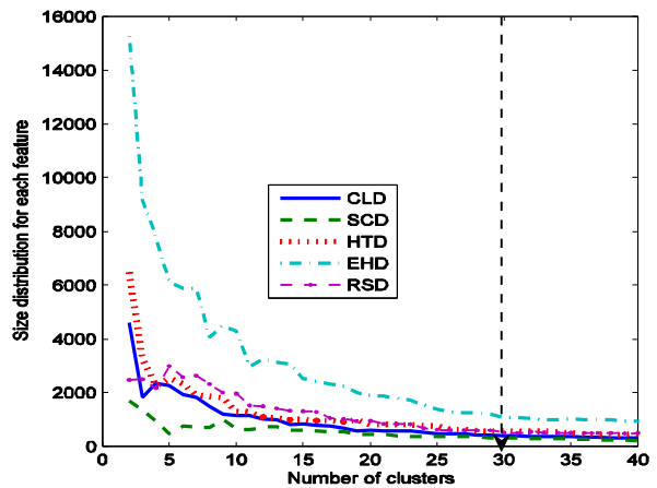
Figure 3. Indexing parameters: the number of clusters
