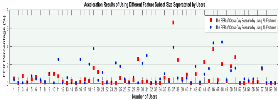
Figure 3: the EER of Using the Walking activity and Utilizing Different Feature Subset Size Separated By Users
