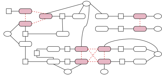
Figure 8: Graph Example
