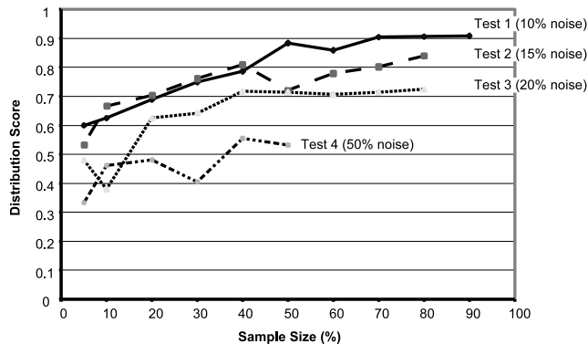
Figure 6: Effect of noise produced by unrelated tuples
