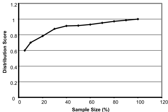
Figure 4: Distribution Scores for relations with the presence of duplicate tuples
