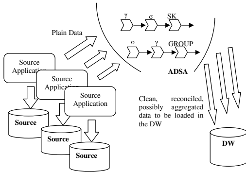
Fig. 1. Architecture Overview
