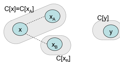
Figure 6: Similarity edges.
