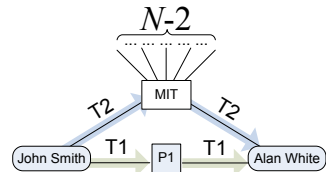
Figure 10: c(p) .
