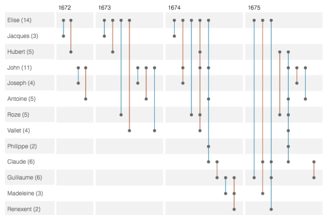
Figure 4: Visualization of a small database sample of business relationships evolving over time for a group of thirteen people using PAOH dynamic hypergraph.
