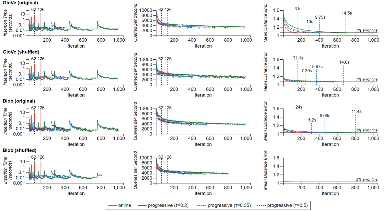
Fig. 1: Benchmark results of online and progressive k -d trees according to datasets (GloVe [41] and Blob) and ordering conditions ( original and shuffled ). FLANN’s online k -d tree (the red line) rebuilt the k -d trees each time the data size doubles, producing insertion times longer than 10 seconds (e.g., leftmost charts at the 62nd and 126th iterations). In contrast, progressive k -d trees (the green, blue, and purple lines) alleviated the spikes in insertion time by spreading the reconstruction load. Our progressive k -d trees yield a small loss in queries per second (middle column), yet with faster convergence to a mean distance error of 7% for the GloVe dataset and 3% for the Blob dataset (rightmost column).
