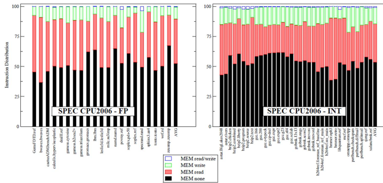
Fig. 1. Memory requirements from SPEC. [1]
