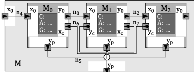
Fig. 2. Erroneous composition resp. refinement of M from the same subcomponents M_i , introducing semantically false connections n_6 and n_7 instead of n_1 and n_3 , which violate the physical semantics of allocating the capacitive loads in correspondence with the real worlds functional interconnections n_0 and n_2 , falsely verifying M.\overline{P} < 20\mu\text{W} .
