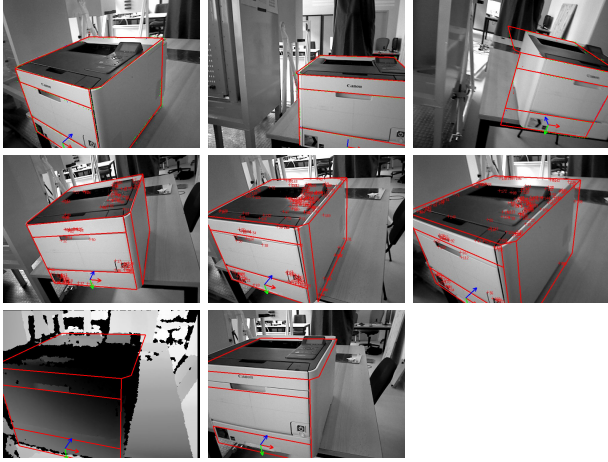
Fig. 5. Top row: edge tracker at frames 282, 564, 684. Middle row: keypoint tracker at frames 150, 200, 228. Bottom row: depth tracker at frame 1 and corresponding color image at frame 1.
