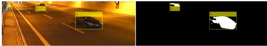
Fig. 8. Blob tracking based on foreground detection
