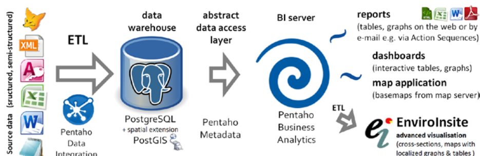
Fig. 1. Architecture of HgIS (arrows represent data flow)
