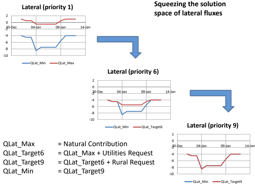
Fig. 3. Solution space squeezing and associated goal stacking for lateral fluxes
