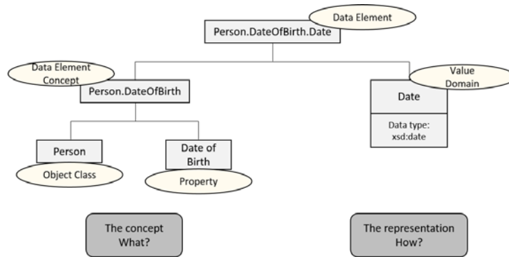
Fig. 1. An example of decomposition of a Common Data Element: Person.DateOfBirth.Date
