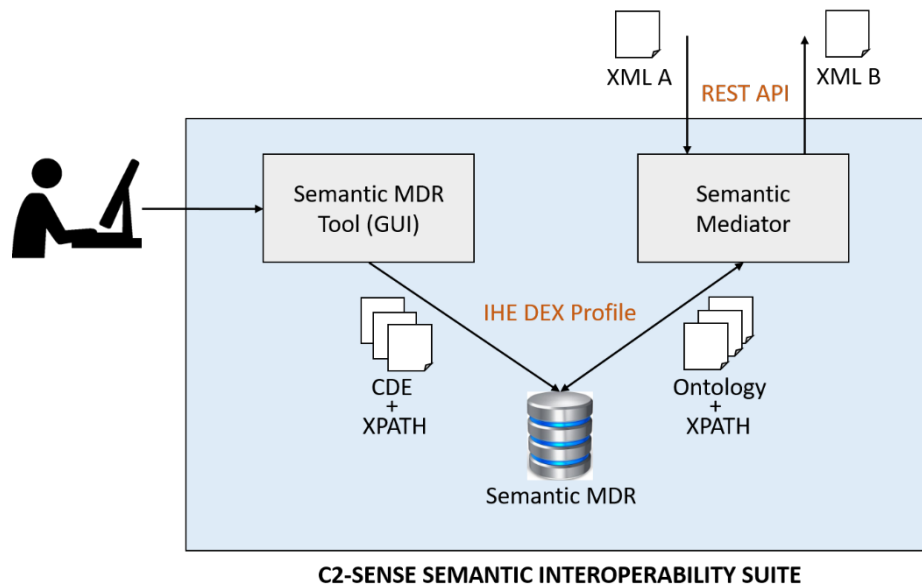
Fig. 2. Architecture of C2-SENSE Semantic Interoperability Suite
