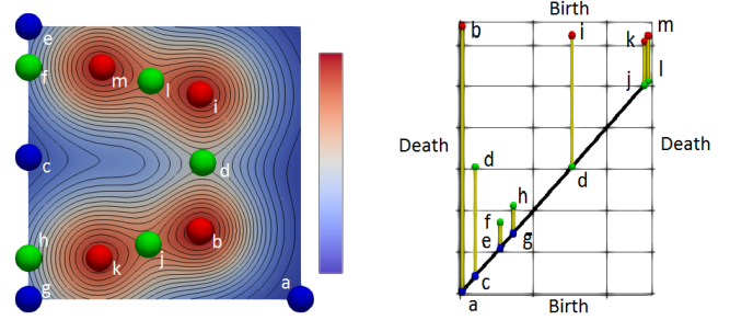
Figure 1: Critical points of a scalar field f defined on a PL 2-manifold (left) and its persistence diagram \mathcal{D}(f) (right). In the persistence diagram, each pair of critical points are represented by a vertical bar (yellow) and their persistence is given by height of the bar.
