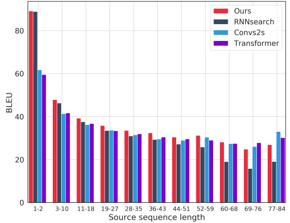
Figure 5: BLEU scores across sentence lengths.
