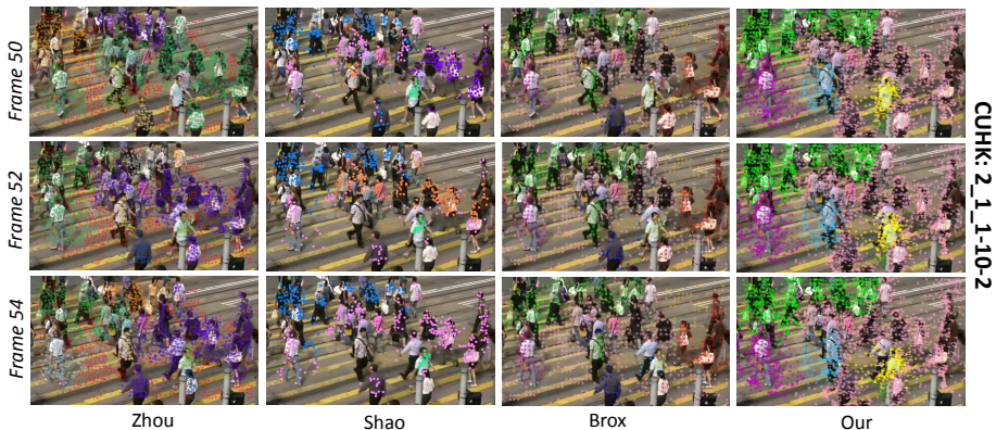
Fig. 1. Segmented motion patterns (or groups segregation) as the crowd evolves in time. The color of point represents the assignment to a group. While groupings are temporally consistent over a set of frames for Brox [2] and Our method. Zhou [3] and Shao [4] fail to maintain consistent groupings between frames.
