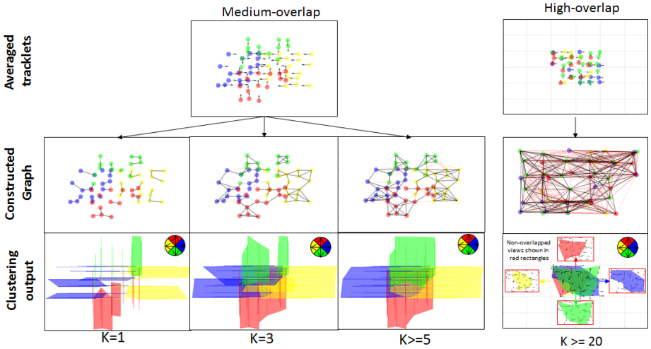
Fig. 3. Visual examples of graph construction for various number of neighbors. First example shows the graph construction for various numbers of k -NN ( first column K=1 , second K=3 , third K=5 ). The second example shows the constructed graph for high motion overlap. For mixed up motion the minimum number of neighbours is 20.
