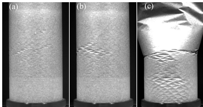
FIG. 1. Snapshots of deformation patterns observed in our experiments. Using the qualitative criteria of Sec. ??, the corresponding deformation processes are classified as (a) far-from-collapse, (b) close-to-collapse, and (c) collapse processes. (a) and (b) show the shell when the deformation stops growing, right before it starts returning to its original undeformed state. (c) shows a shell after catastrophic failure. The upper section of the shell has collapsed against a protective glass cylinder surrounding the silo.
