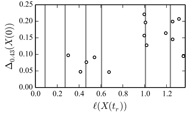
FIG. 7. Arc length coordinate of the points X(t_r) for each FFC trajectory X versus \Delta_{0.43}(X(0)) . Vertical lines mark the coordinates of transition points of the trajectory X^R .
