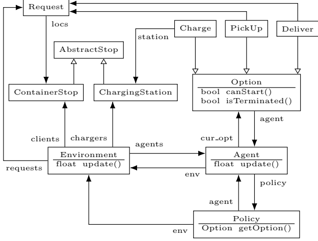
Figure 3. A simplified class diagram of the SULFR interface. Only key methods are included: update() , called at all simulation time step to update the state of the agents and the environment; isTerminated() , also called at every time step, checking for termination condition of the options; canStart() , used to filter available options when the previous one has ended. Policies have access to the whole state of the agents and the environment.
