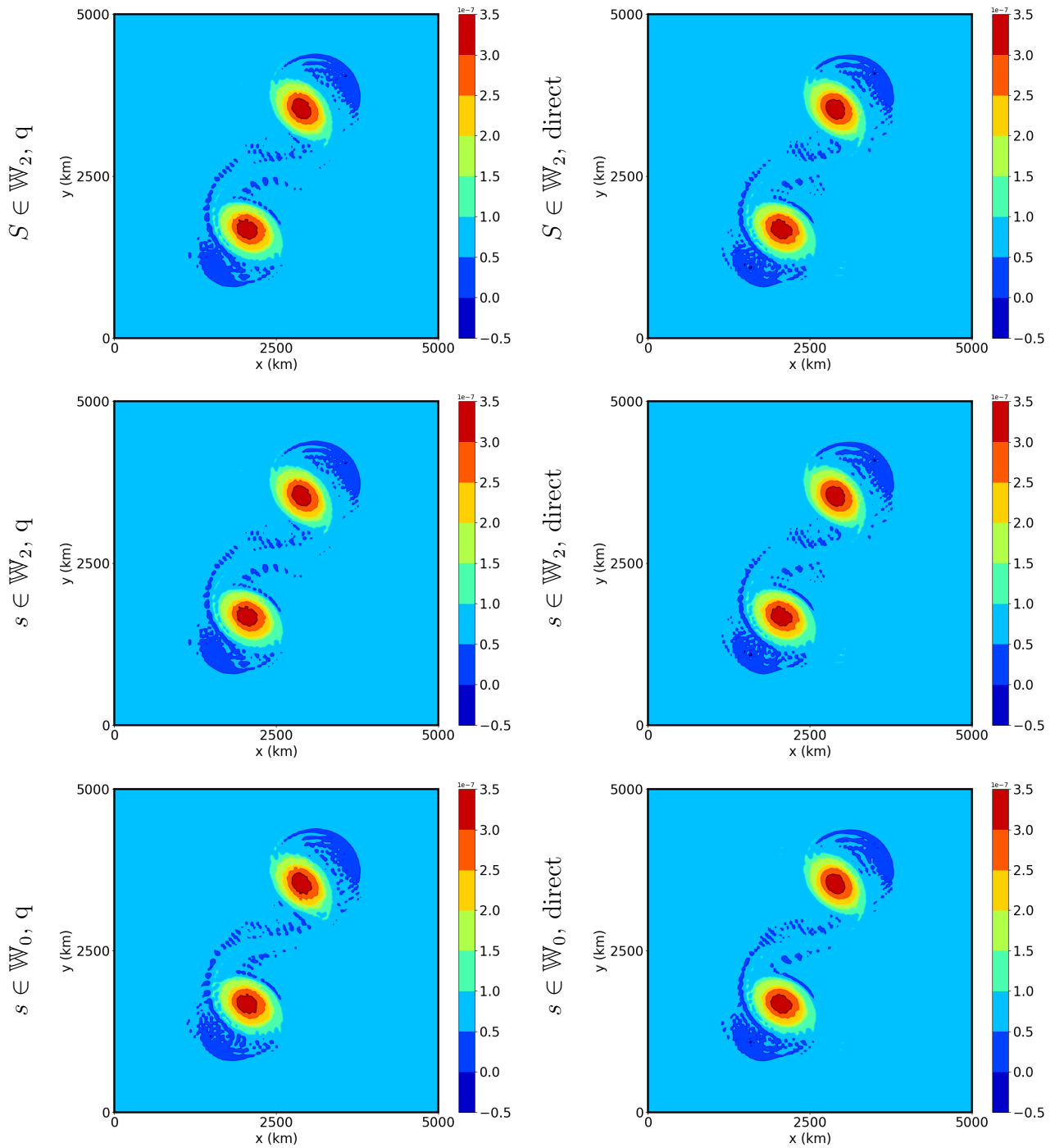
Figure 6: The potential vorticity q at N = 250 for the double vortex test case for all six variants. Small scale features have developed following the path of the vortices, although the main vortex cores remain coherent. There is little difference between the six variants.
