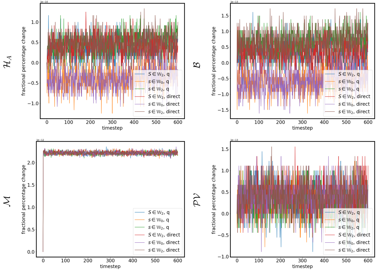
Figure 10: Convergence properties for \mathcal{M} , \mathcal{B} , \mathcal{H}_A and \mathcal{PV} in the thermal instability test case, shown for all six variants. The fractional change (\frac{x-x_0}{x_0} * 100) in the relevant quantity versus the time step is plotted. As in Figure 5, all variants are conserving \mathcal{M} , \mathcal{B} , \mathcal{H}_A and \mathcal{PV} to machine precision, albeit with a strange (and still unexplained) jump in mass in the first time step for all variants.
