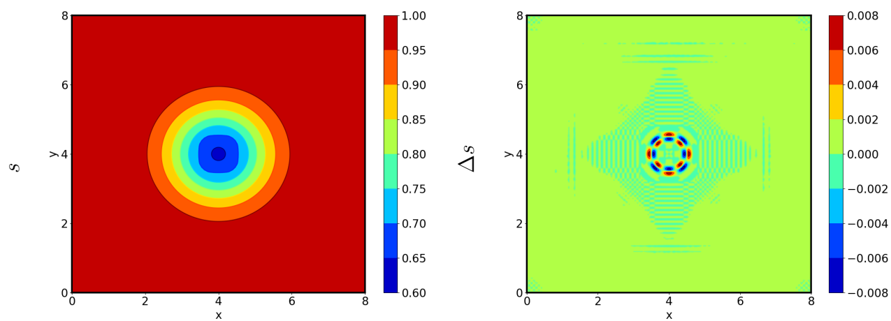
Figure 8: The initial (left) and perturbation (right) values for the buoyancy s in the thermal instability test case. Recall that l = 4 , and the perturbation is localized to a small ring of the domain.
