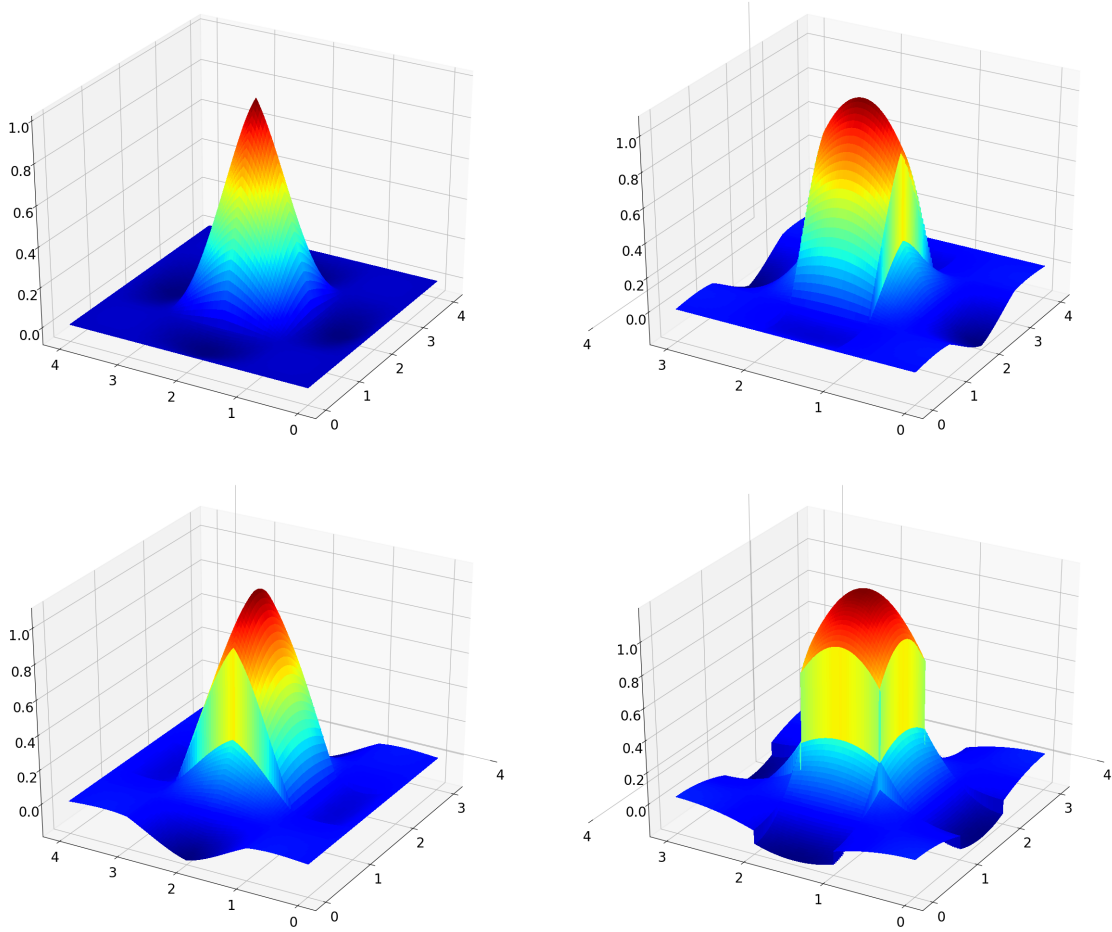
Figure 1: Basis functions for the \mathbb{W}_0 (upper left), \mathbb{W}_1 ( x component in upper right, y component in lower left) and \mathbb{W}_2 (lower right) spaces of the MGD_3 family. Here the element width and basis functions have been normalized to unity. Note that all of the basis functions in a given space are identical, and that the basis functions are not localized to an element or a pair of neighboring elements, but instead have extended support (although they remain local).
