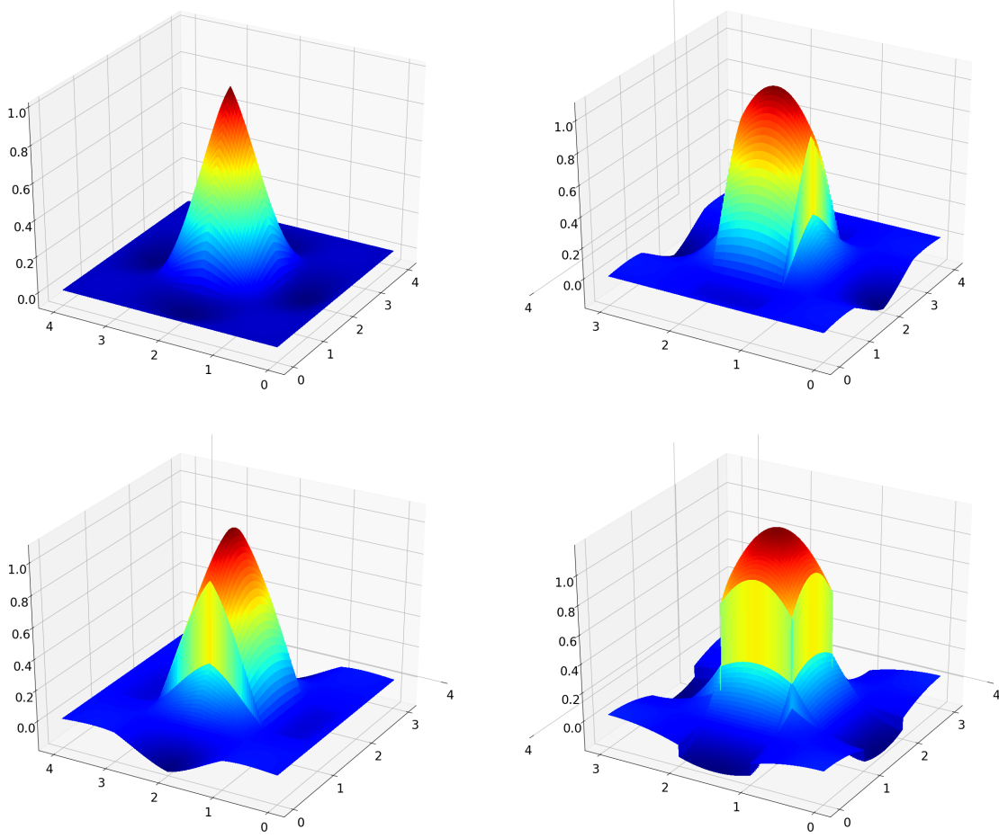
Figure 1: Basis functions for the \mathbb{W}_0 (upper left), \mathbb{W}_1 ( x component in upper right, y component in lower left) and \mathbb{W}_2 (lower right) spaces of the MGD_3 family. Here the element width and basis functions have been normalized to unity. Note that all of the basis functions in a given space are identical, and that the basis functions are not localized to an element or a pair of neighboring elements, but instead have extended support (although they remain local).
