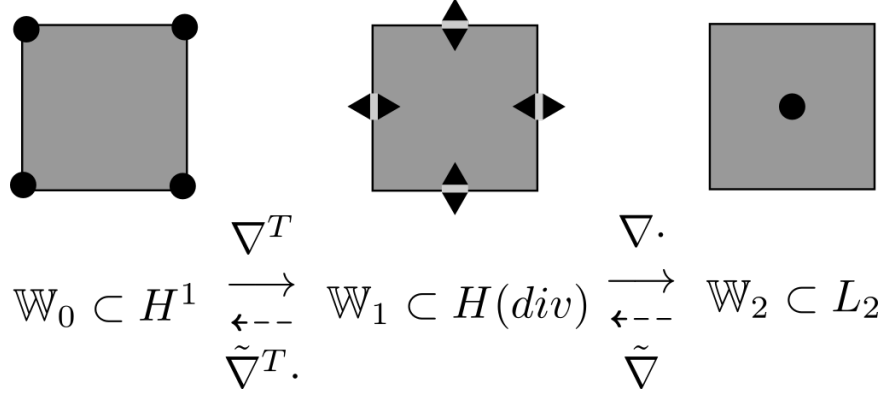
Figure 2: Compatible Galerkin spaces \mathbb{W}_0 , \mathbb{W}_1 and \mathbb{W}_2 in 2D for the MGD_n family. Solid lines indicate strong operators ( \nabla^T , \nabla \cdot ), while dashed lines indicate weak operators ( \tilde{\nabla} , \tilde{\nabla}^T ). The degrees of freedom are illustrated for the MGD_n family, which are also correct for the lowest order Q_r^- \Lambda^k /mimetic spectral element and odd-order isogeometric analysis families.
