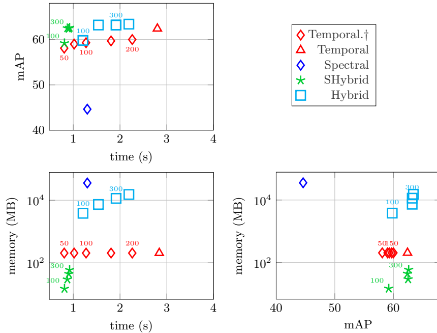
Fig. 5. Positioning of different methods on time (s) - memory (MB) - performance (mAP) axes. We show mAP vs. time, memory vs. time, and memory vs. mAP on \mathcal{R}Oxford + \mathcal{R}1M . Methods in the comparison: temporal for 20 iterations, truncated temporal for 20 iterations and shortlist of size 50k, 75k, 100k, 200k and 300k, spectral (FSRw) with r = 5k , hybrid with r \in \{100, 200, 300, 400\} and 5 iterations, sparse hybrid with 99% sparsity, r \in \{100, 200, 300, 400\} and 5 iterations. Text labels indicate the shortlist size (in thousands) for truncated temporal and rank for hybrid. Observe that the two plots on the left are aligned horizontally with respect to time, while the two at the bottom vertically with respect to memory.
