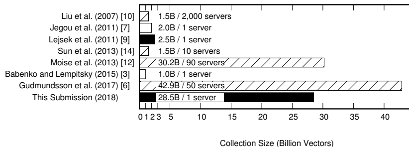
Fig. 1. The largest experimental collections reported in the literature. Black bars represent results using the NV-tree. Shaded bars represent multi-server configurations.
