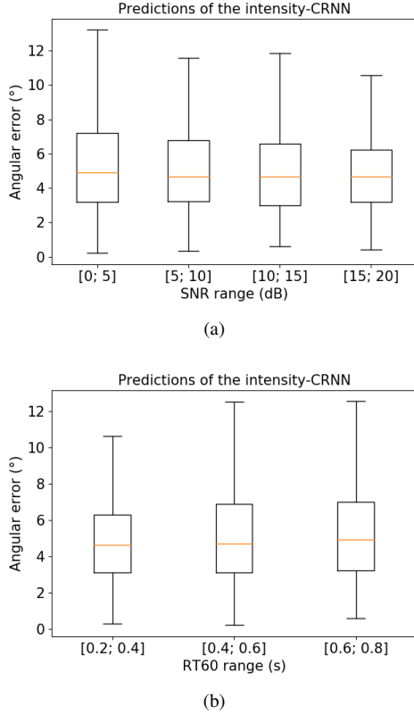
Fig. 10. Boxplots of the angular errors ( ^{\circ} ) for all sequences of the single-source DoA estimation as a function of (a) the SNR and (b) the RT_{60} , on signals generated from simulated SRIRs. The boxes show the first and third quartiles in black and the median in orange. The lower ends of the whiskers correspond to the lowest data still within 1.5 interquartile range (IQR) of the lower quartile, and similarly the higher ends of the whiskers correspond to the highest data within 1.5 IQR of the upper quartile.
