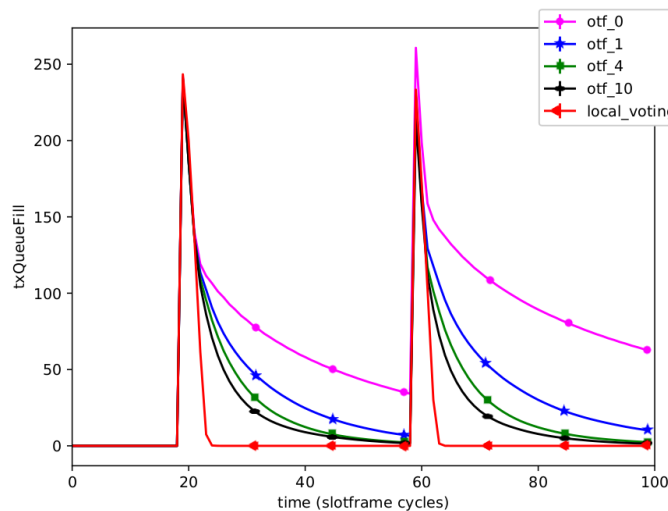
FIGURE 13 Queue usage during a simulation for different SF0 thresholds and when using a Local Voting scheme for load balancing. Reproduced from (10).
