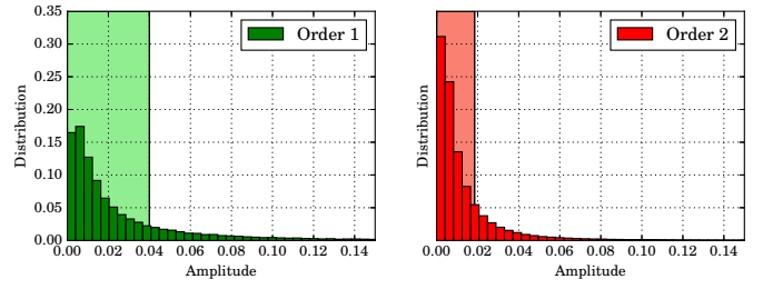
Fig. 5: Histogram of \hat{F}_1 amplitude for first and second order coefficients. The vertical lines indicate a threshold that is used in Subsection 4.3 to sparsify \hat{F}_1 .
