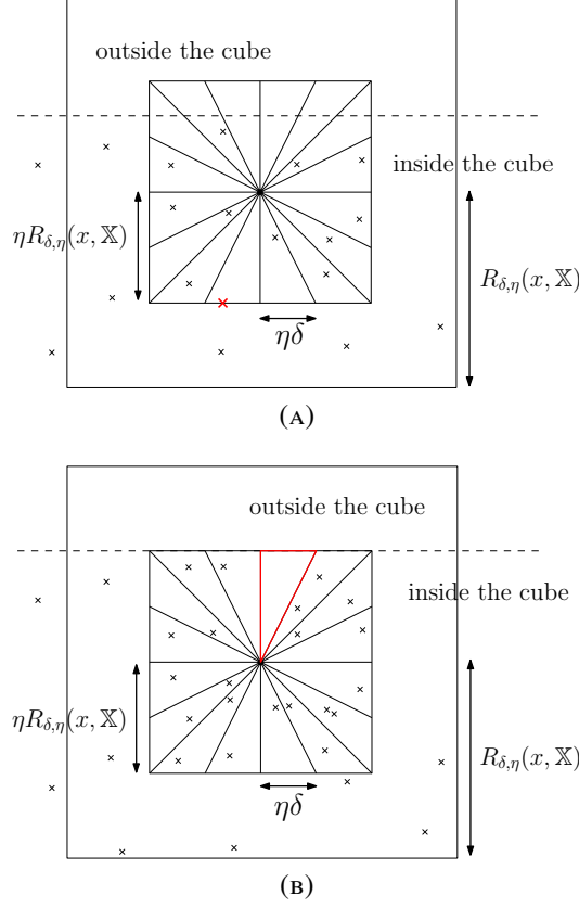
FIGURE 3. Illustration of the definition of R := R_{\delta, \eta}(x, \mathbb{X}) for some two point clouds \mathbb{X} . The dashed line indicates the boundary of [0, 1]^d . In Figure 3a, the radius R is such that there is a point (indicated in red) on C_j^\delta(x, R) . In Figure 3b, there is a cone A_j^\delta(x, R) , indicated in red, for which C_j^\delta(x, R) is on some face of the cube [0, 1]^d .
