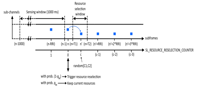
Fig. 3. Semi-persistent scheduling (SPS) according to 3GPP Rel.14.
