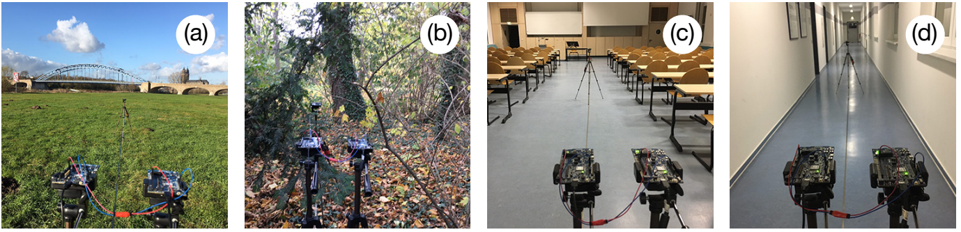
Fig. 2: Experimental environments: (a) is an open field park with line-of-sight (LoS) transmission, (b) is a forest with blocked LoS, (c) is a classroom located in a university building, and (d) is a corridor at the same university building. Environment (c) and (d) include random people movement during experimentation.
