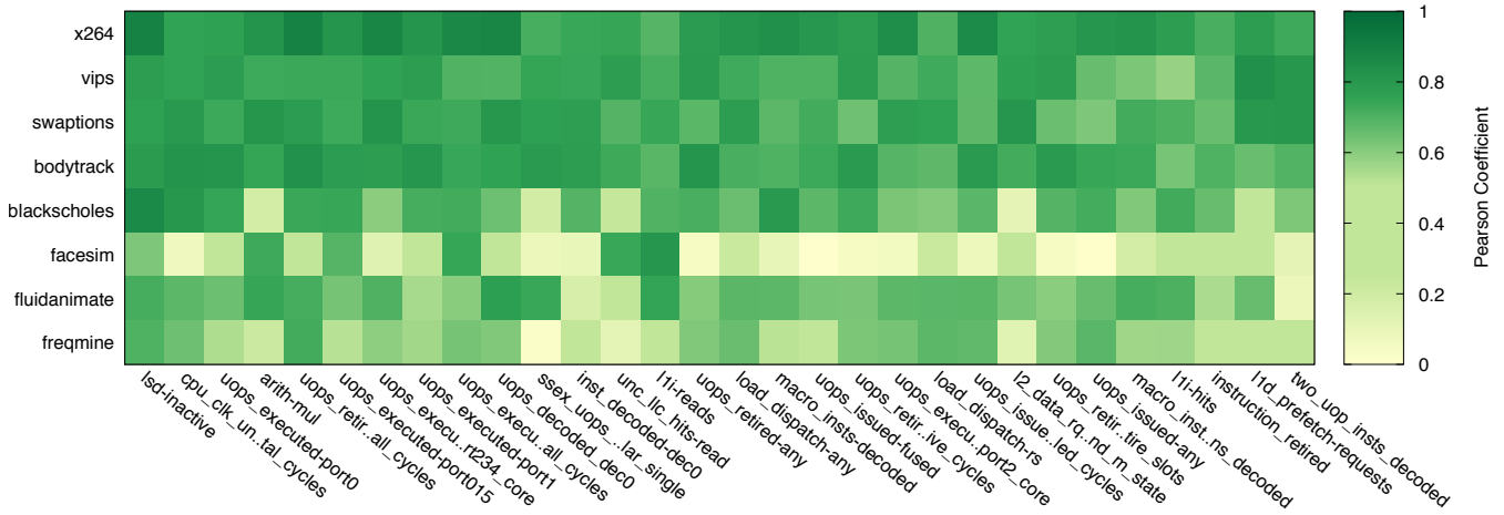
Figure 3: Pearson coefficients of the Top-30 correlated events for the PARSEC benchmarks on the Intel Xeon W3520.
