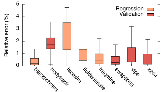
Figure 5: Relative error distribution of the PARSEC benchmarks on the Xeon processor ( P_{idle} = 92 \text{ W} ).
