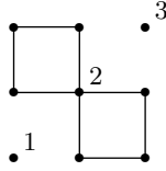
FIGURE 2. An associative operation on X_3 that is not quasitrivial
