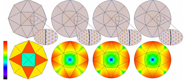
Fig. 5. Determinant of Jacobian. From left to right: ODT mesh ( n=1 ), then curved ODT meshes with order 2, 3 and 5 respectively, showing increasing continuity across elements. Bottom: determinant of the Jacobian in the domain visualized with a rainbow colormap.
