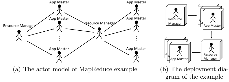
Fig. 4. The MapReduce example
