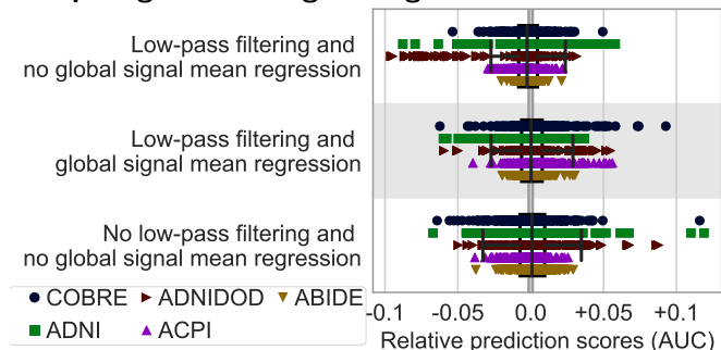
Figure A9: Temporal signal filtering strategies on prediction accuracy (AUC) for five rs-fMRI datasets: Distribution of relative prediction scores showed no big differences across three filtering strategies: lowpass filter and no global signal regression, lowpass filter and global signal regression, no lowpass filter and no global signal regression.
