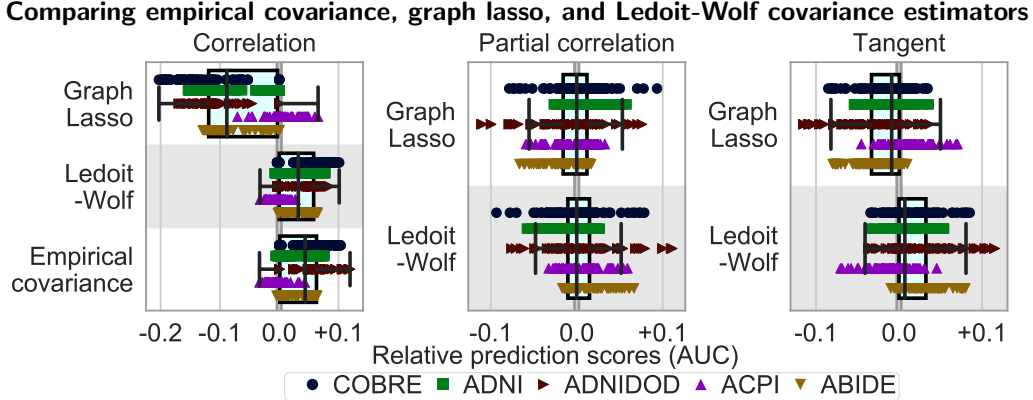
Figure A11: Impact of covariance estimator, for the different connectivity parametrizations: Marginal distribution of relative prediction scores per connectivity method across covariance structures for all rest-fMRI datasets. This is obtained by considering the good choices in dimensionality as studied in the main figures. Overall, using empirical covariance instead of Ledoit-Wolf shrinkage yield minor difference in prediction performances; note that partial correlation and tangent parametrization require the use of shrinkage. Graph lasso tends to perform lower compared with other estimators.
