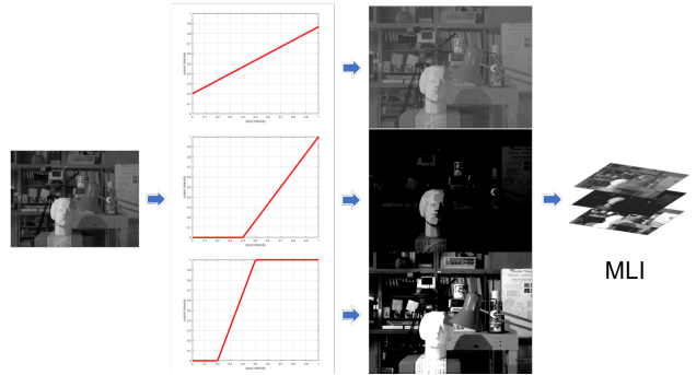
Fig. 3. Using SAT function with different contrast bands to generate a multi-layered image representation (MLI).
