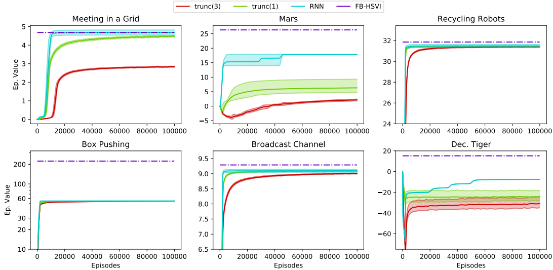
Figure 3: Comparison of different structures used to represent histories.
