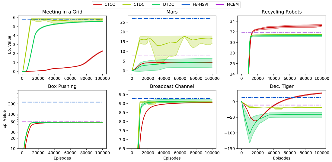
Figure 5: Comparison of the three paradigms for T = \infty .
