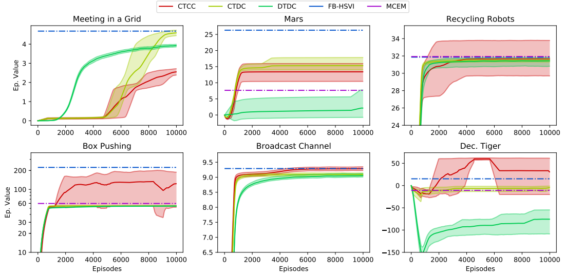
Figure 4: Comparison of the three paradigms for T = 10 .
