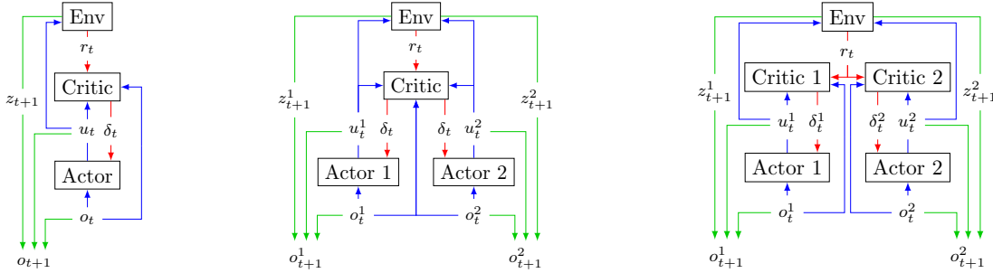
Figure 1: Best viewed in color. For each paradigms—(left) CTCC; (center) CTDC; and (right) DTDC—we describe actor-critic algorithmic schemes. We represent in blue, green and red arrows: forward control flow; the aggregation of information for the next time step; and the feedback signals back-propagated to update all parameters, respectively.
