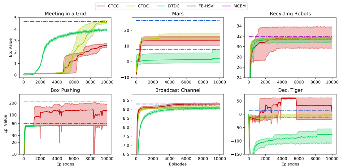
Figure 4: Comparison of the three paradigms for T = 10 .
