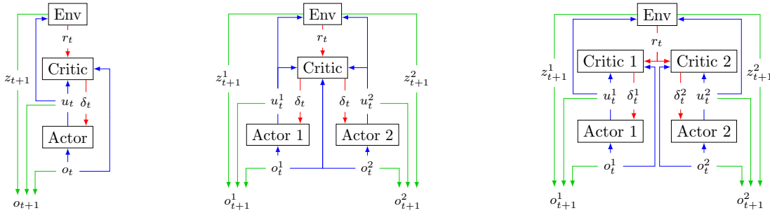
Figure 1: Best viewed in color. Actor-critic algorithmic schemes in a two-agent setting for paradigms: (left) CTCC; (center) CTDC; and (right) DTDC. In all figures, blue arrows represent forward control flow, green arrows show the aggregation of information for the next time step, and red arrows are the feedback signals back-propagated to update all parameters.
