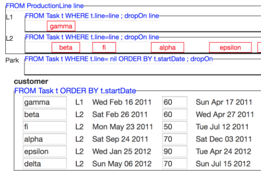
Fig. 2. Fully declarative user interface featuring advanced interaction like drag and drop
