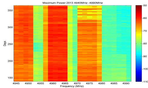
Fig 5. 4.945 – 4.99 GHz Broadband Public Safety during 2013
