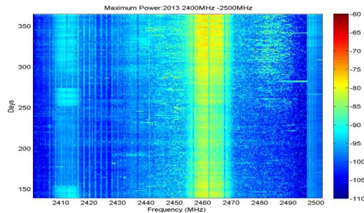
Fig 4. 2.4 GHz Band during 2013
