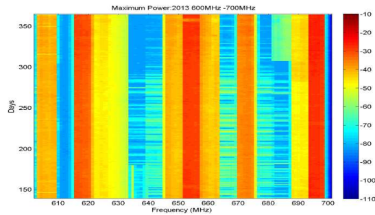
Fig 3. 600 MHz television bands during 2013
