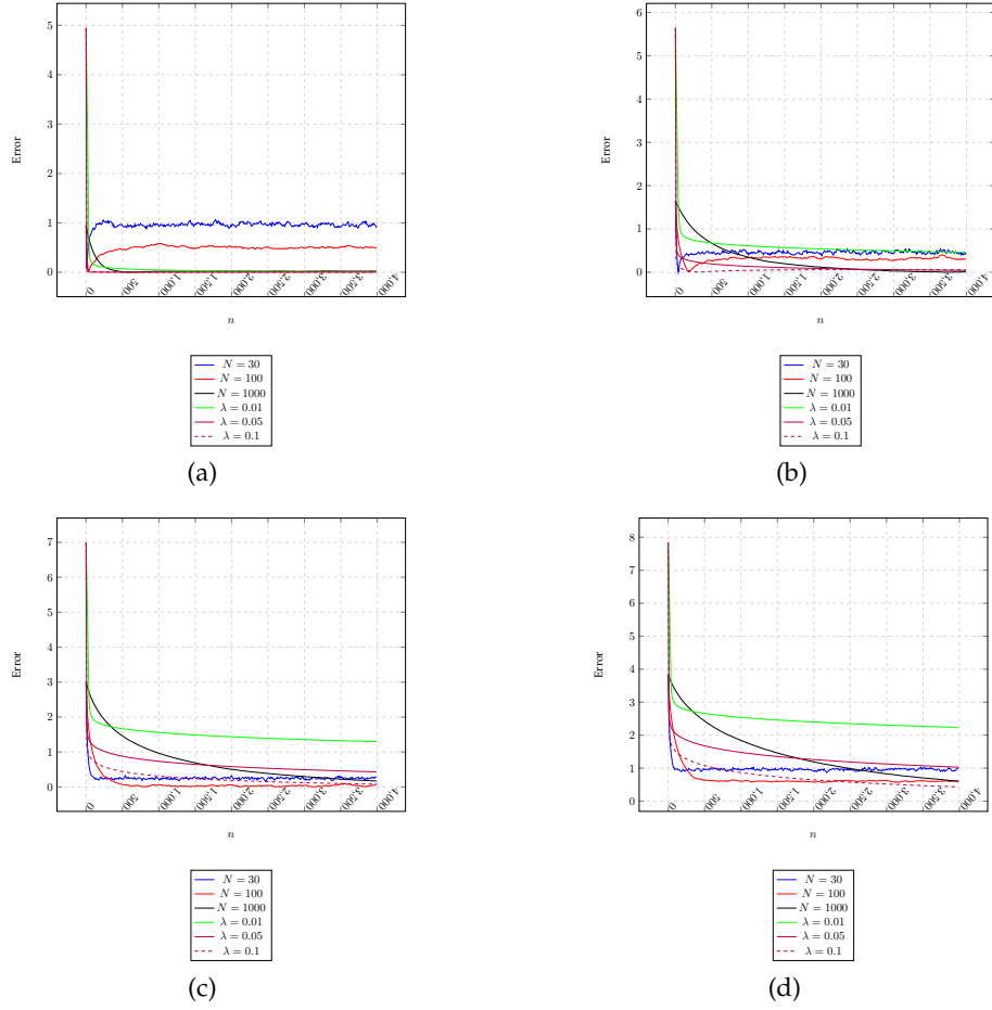
Fig. 4. This figure depicts the variation of the estimation error with time n for the quantile of 95% for the DQE ( N = 30 , N = 100 and N = 1000 ) and for the EWSA ( \lambda = 0.01 , \lambda = 0.05 and \lambda = 0.1 ) for (a) uniform distribution, (b) normal distribution, (c) exponential distribution, (d) Chi – Square distribution.
