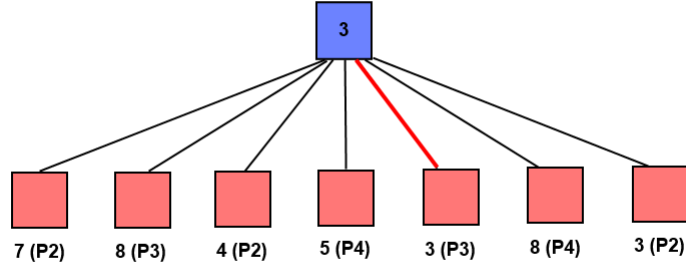
Fig. 1: The operation of a single level of the Best-Reply Search. The scores that are reported have the opponent’s player number listed next to them (in parenthesis) to assist in the clarification.
