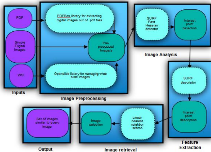
Fig. 2. Workflow diagram of the proposed methodology (Magenta boxes correspond to input/output, light green to processing steps and dark green refers to intermediate objects)
