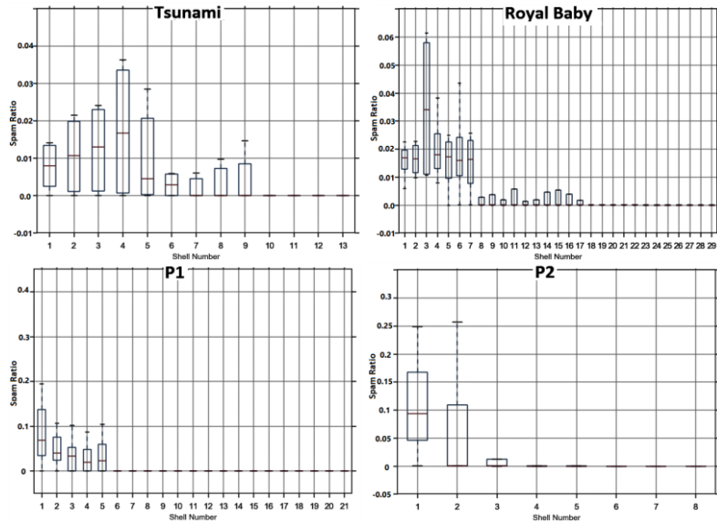
Fig. 2. Box plot representing the probability distribution of the percentage ratio between the spam count in each k -shell to the shell size. The x-axis represents the ( k ) value of the k -shell, and the y-axis represents the percentage ratio of the number of spam accounts in a given k -shell to the number of nodes in the same k -shell.
