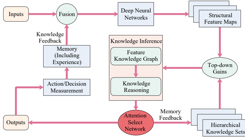
Fig. 1: General framework of cognition-based deep learning
