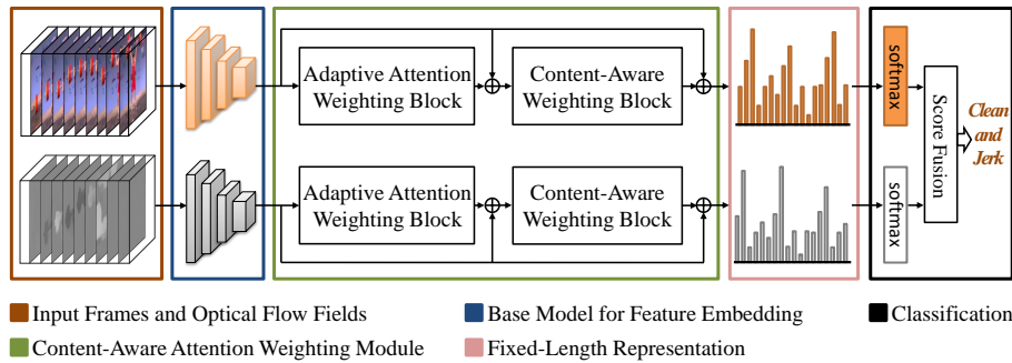
Fig. 2. Content-aware attention network. The inputs are video frames and optical flows. First, they are embedded by a CNN (base model). Then, the extracted features are aggregated by the proposed content-aware attention weighting module, and a fixed-length representation can be obtained. Finally, we use this representation to classify the input video, and adopt score fusion to obtain the prediction of the video.
