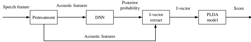
Fig.1. DNN-based Speaker Identification System Flow Chart
