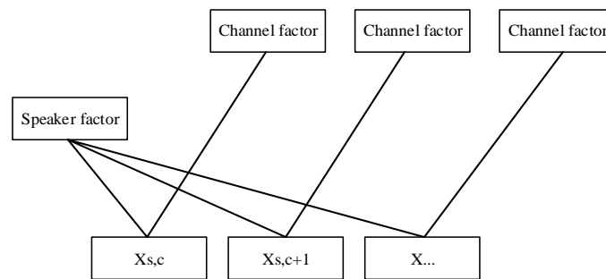
Fig.5. RBM-PLDA
