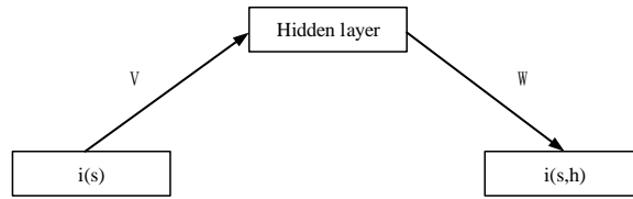
Fig.3. RBM Pre-training
