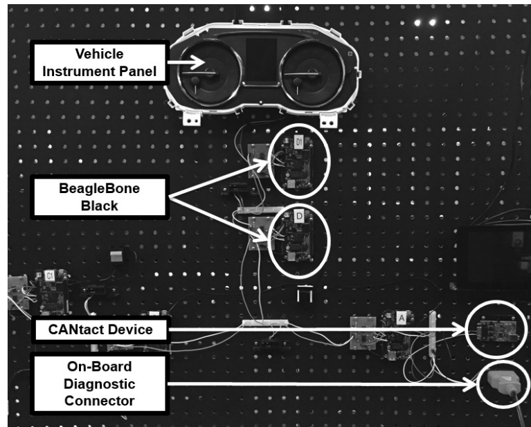
Figure 1. Automobile CAN bus emulation testbed.
