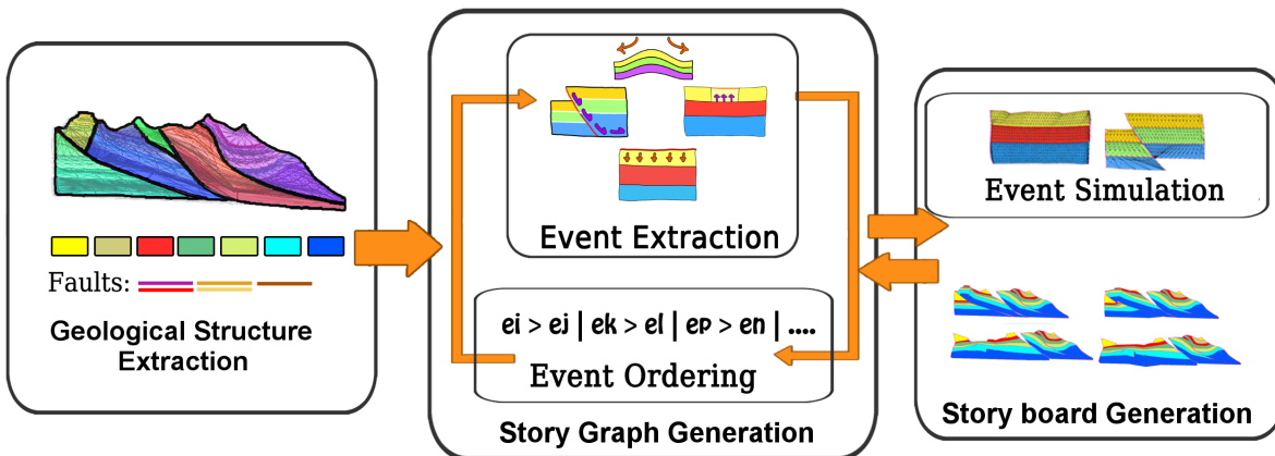
Figure 3: Process Overview (from left to right): (i) input sketch analysis for geological structure extraction; (ii) generation of branching geological story graph; (iii) Undo event simulation and storyboard sketch generation.
