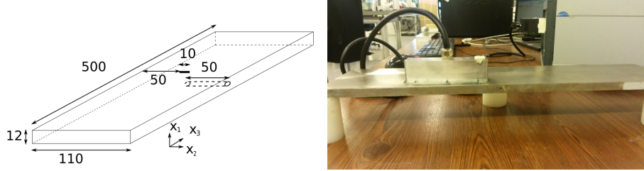
Figure 7: Left: scheme of the plate with defects. Right: experimental setup.
